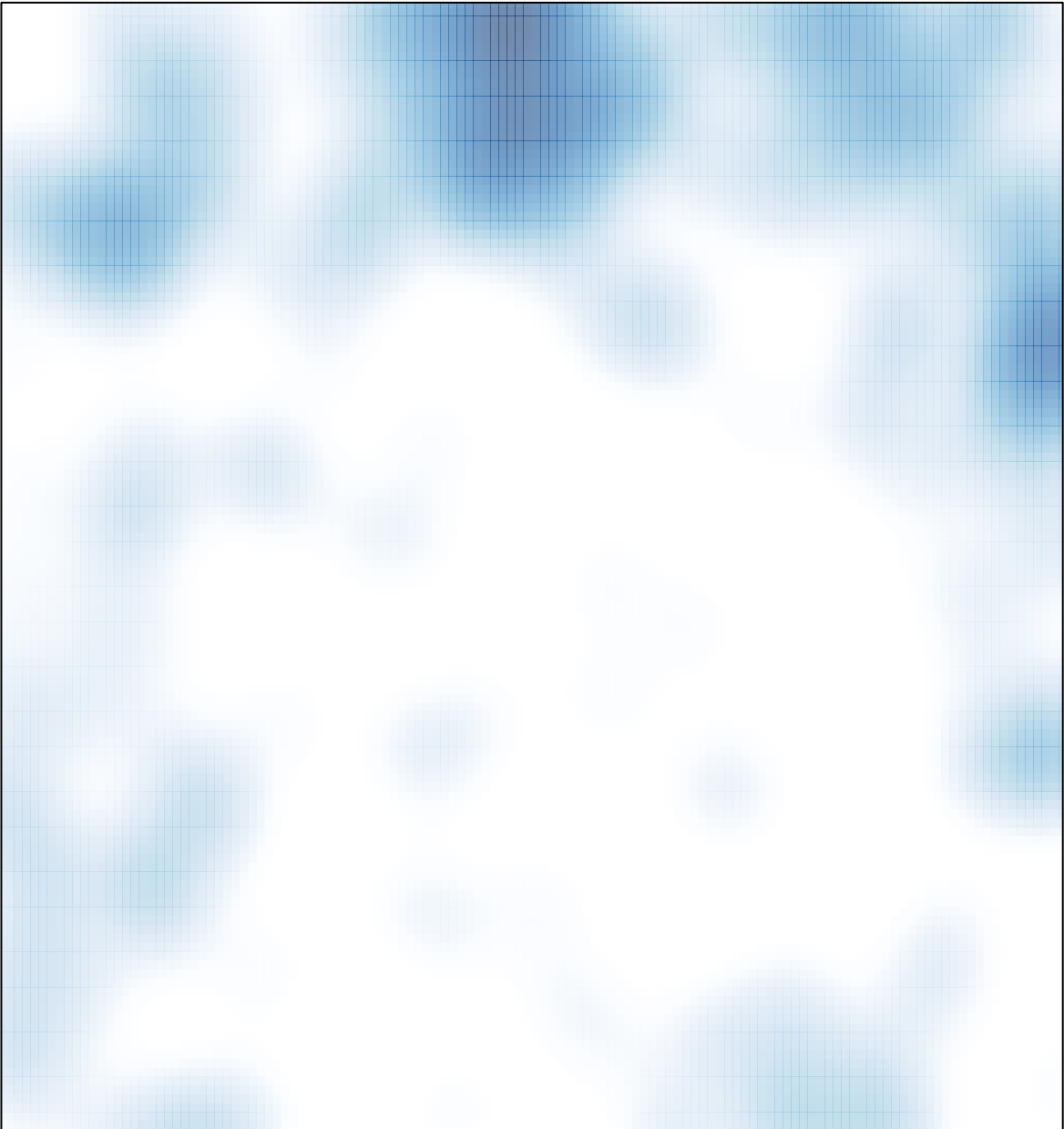
# features = 316 , max = 5
